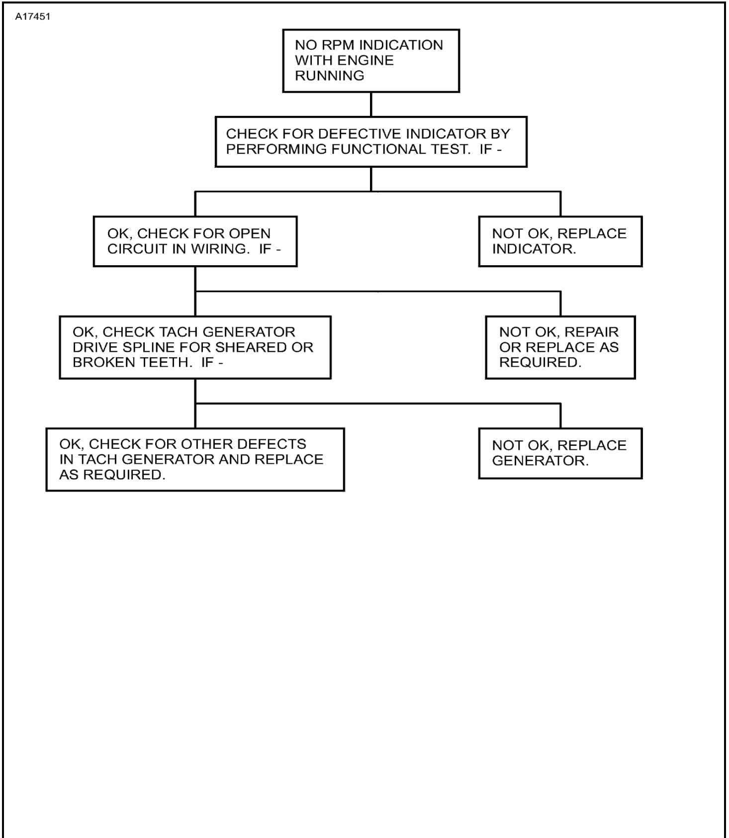
Figure 101 : Sheet 1 : Propeller RPM Indicator Troubleshooting Chart
